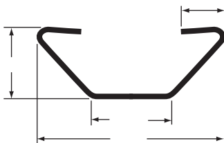
1" ROOF BOW, 18 GA, 80GR, 98.75"
