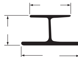
ROOF BOW, CAMBERED, ALUM, 98.5"
