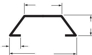
ROOF BOW, ANTI-SNAG, ALUM, 98.5"
