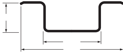
3.44" ROOF BOW, HAT STYLE, 98.88"
