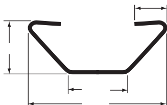
ROOF BOW, ANTI-SNAG, ALUM, 99"
