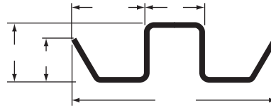
ROOF BOW, 16 GA STEEL, 99.125" L
