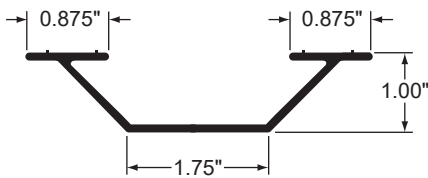
Aluminum Anti-Snag Cambered
