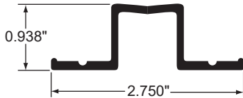
ROOF BOW, 100" LONG
