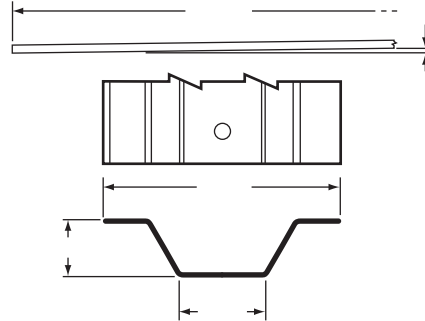
ROOF BOW, STEEL, 99.125"
