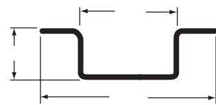
HAT STYLE ROOF BOW, 16 GA, 99"
