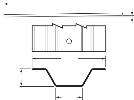
ROOF BOW, STEEL, 91.8"
