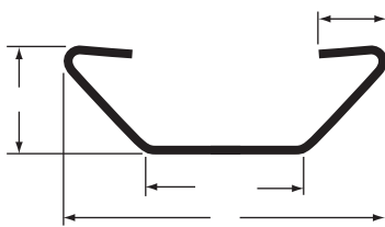
ROOF BOW, ANTI-SNAG, 99"
