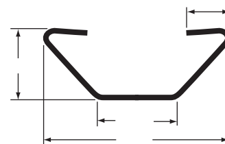
ROOF BOW, CAMBERED, ALUM, 97 1/8"
