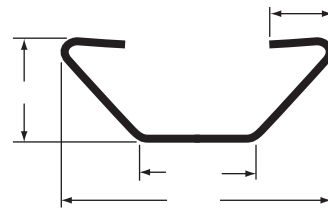
ROOF BOW, 18 GA GALV STEEL, 93.75"
