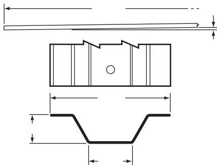
3/4" ROOF BOW, ARCH, STEEL 98.62"
