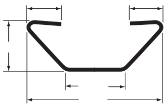
ROOF BOW, ANTI-SNAG, 99.375"
