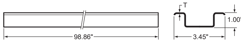
ROOF BOW, 3.45" W, 98.86"
