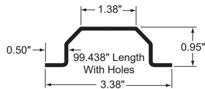
Utility Steel Cambered Roof Bow
