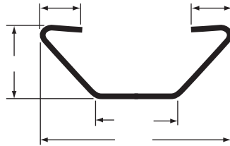
2.675" ROOF BOW, 18 GA, 96"
