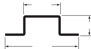
ROOF BOW, 98.5" L
